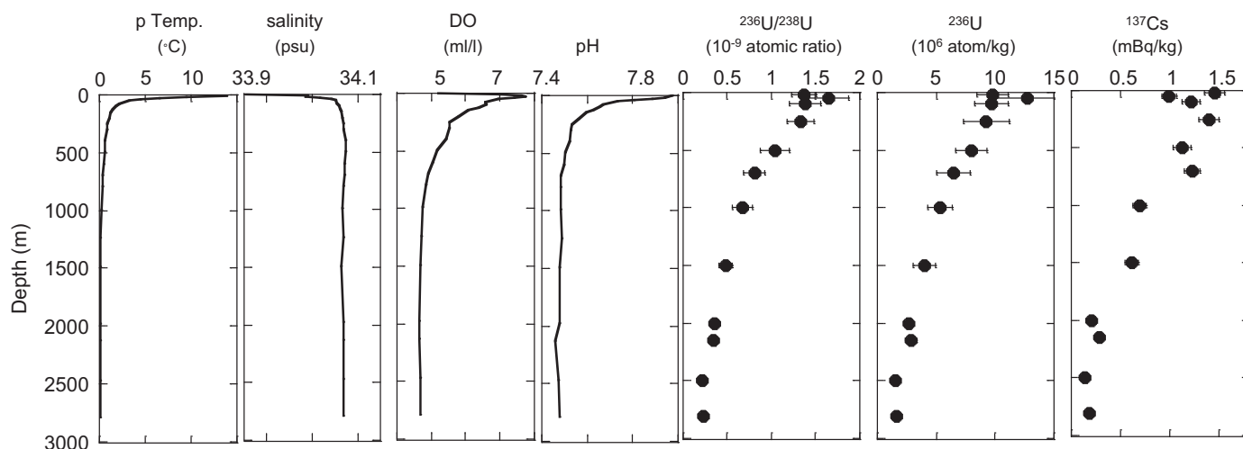
Fig. 2. Depth profiles of ^{236}\text{U}/^{238}\text{U} atom ratio and the concentration of ^{236}\text{U} (atom/kg) together with ^{137}\text{Cs} (mBq/kg) in the water column at the CR58 site. Error bars are one standard deviation. Potential temperature ( ^{\circ}\text{C} ), salinity (psu), pH (SWS scale 25^{\circ}\text{C} ) and dissolved oxygen (ml/l) data are also shown.
