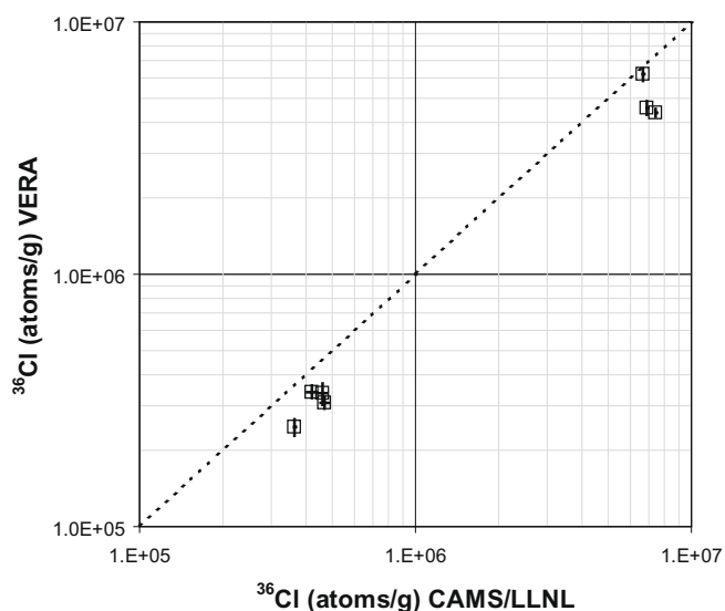
Fig. 4. ^{36}\text{Cl} concentrations measured at VERA compared to values measured at the CAMS facility [6,7]. There is a general agreement, but apparently an offset of \sim 25\% . The reason is under investigation.
