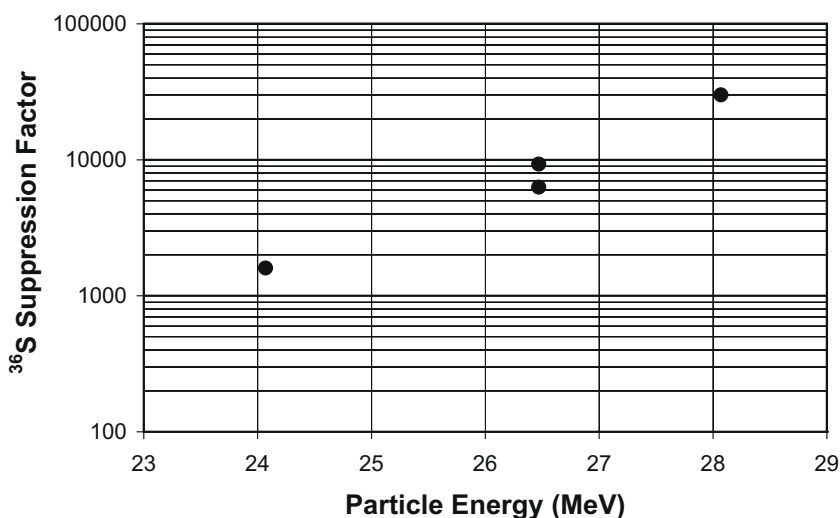
Fig. 2. The ^{36}\text{S} suppression grows strongly with energy. The points were obtained for the 7+ charge state at 3, 3.3, and 3.5 MV terminal voltage, respectively.
