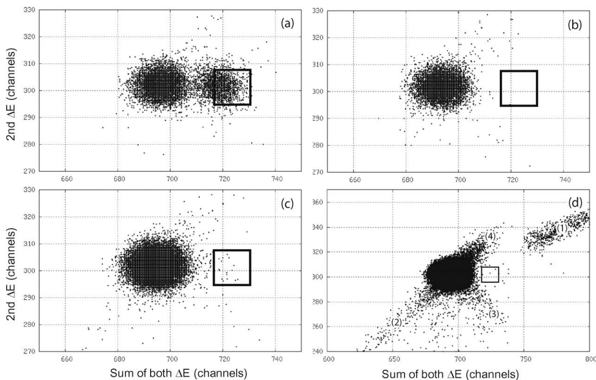
Fig. 1. Typical spectra obtained within 5 min for a standard (a), a blank (b), a true sample (c), and a blank without chemical sulfur suppression (d). 1 MeV energy loss corresponds to 40 channels. The frame indicates the ^{36}\text{Cl} integration region. The tails in (d) are: pulse pile-up (1), larger energy loss, i.e. nuclear stopping, in the entrance window (2), larger energy loss in anode 1 (3), larger energy loss in anode 2 (4). Note the different scale in (d).
