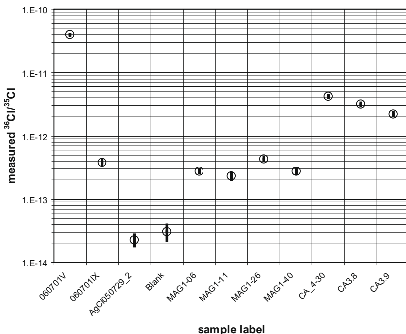
Fig. 3. ^{36}\text{Cl}/^{35}\text{Cl} ratios measured at VERA, after sulfur-proportional background subtraction. 060701V: normalization standard (nom. 4.0 \times 10^{-11} ); 060701X: diluted standard (nom. 4.0 \times 10^{-13} ); AgCl050729_2: precipitated silver chloride (Merck, pA); Blank: process blank; "MAG..." and "CA..." are exposure dating samples from Italy [6], and Iran [7], respectively.
